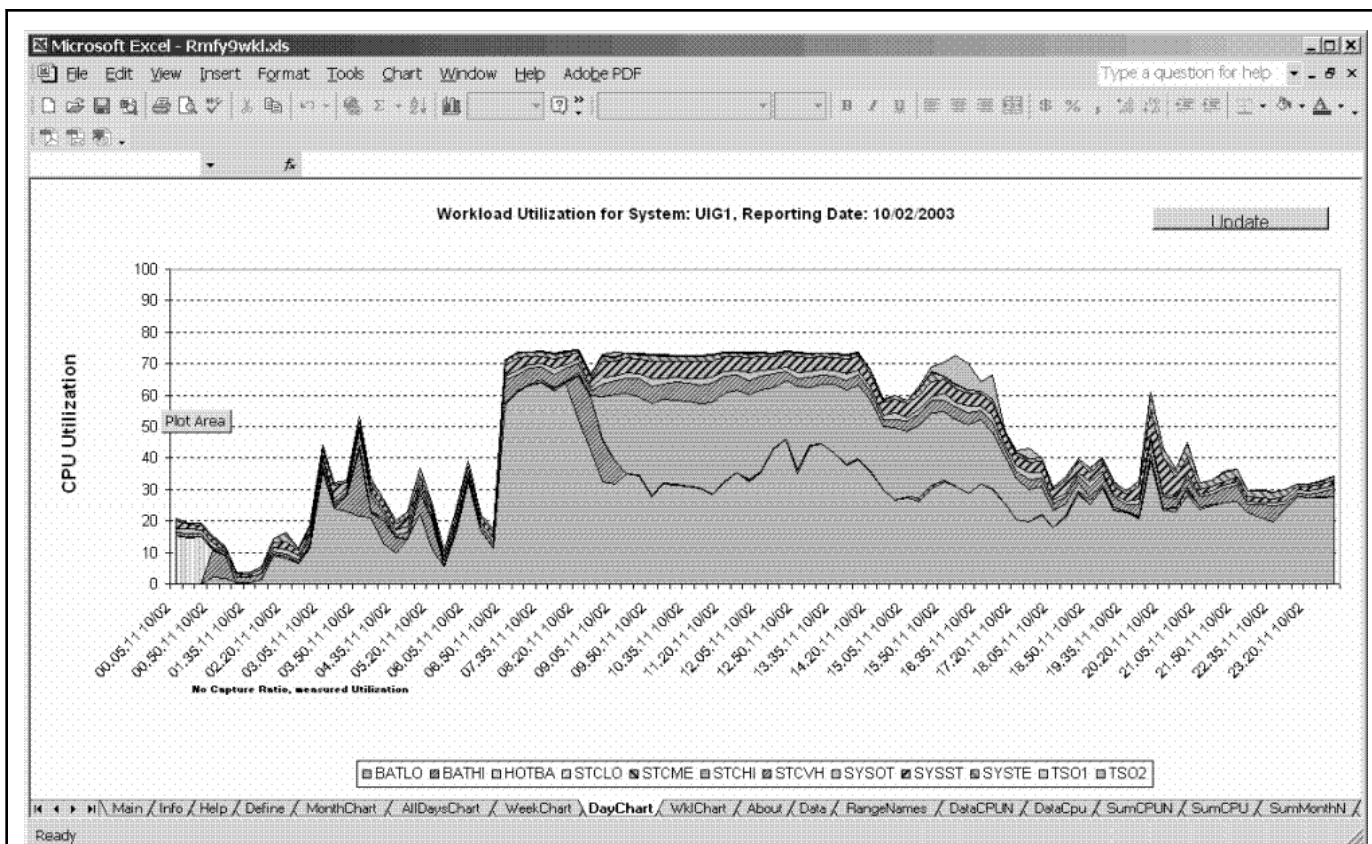
Figure 51. Spreadsheet - CPU utilization for selected workloads
