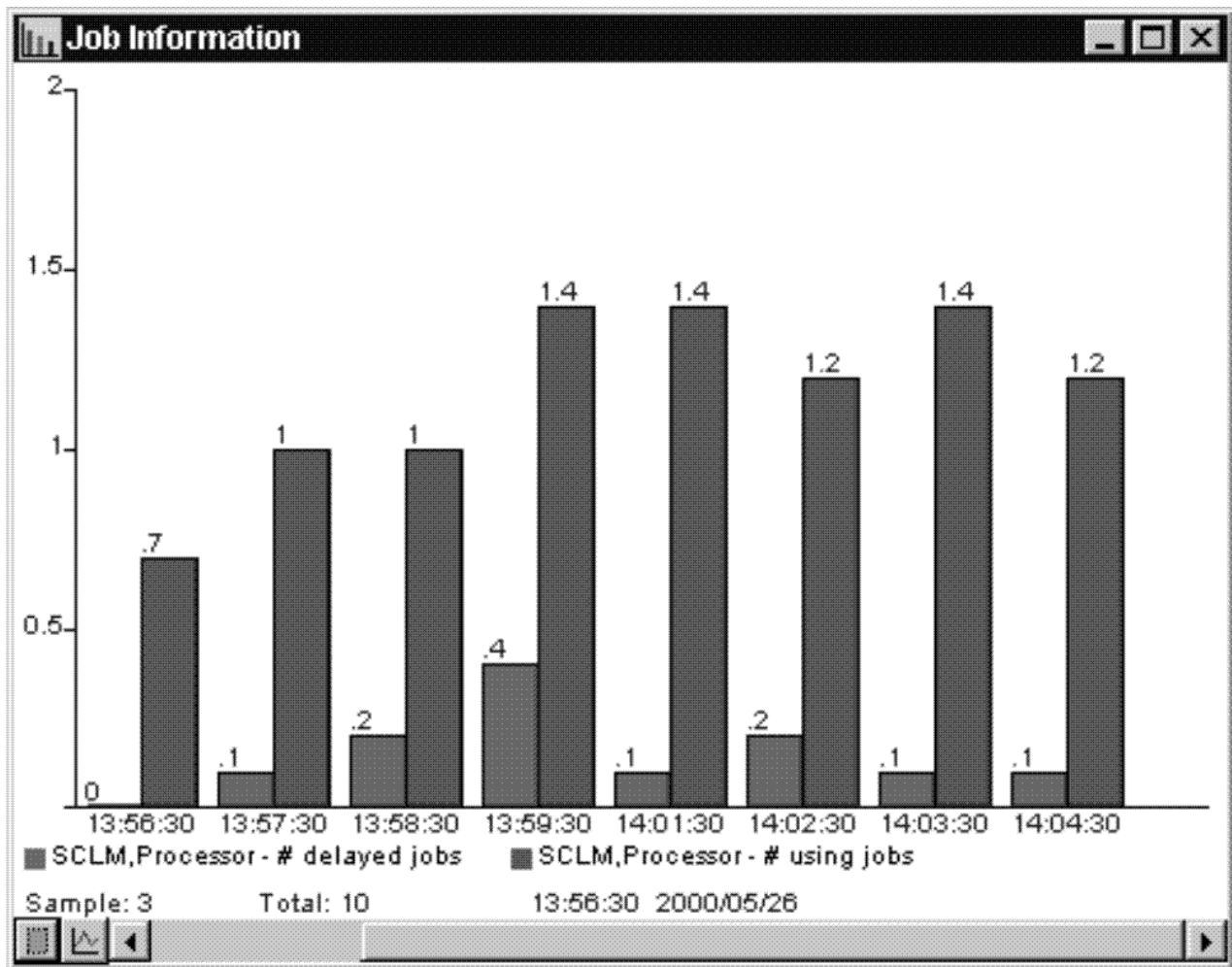
Figure 75. Sample DataView
