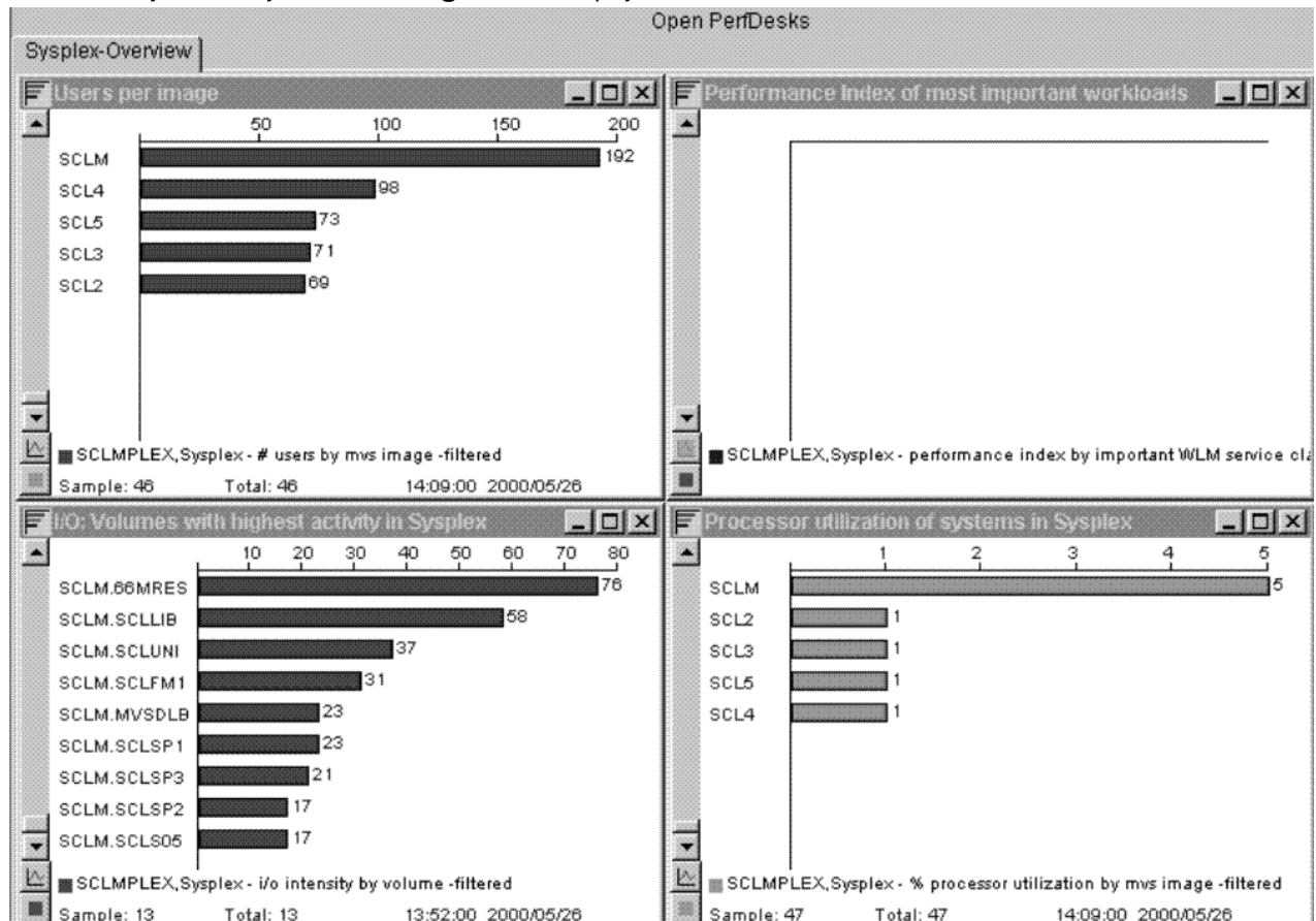
Figure 72. Initial DataViews
