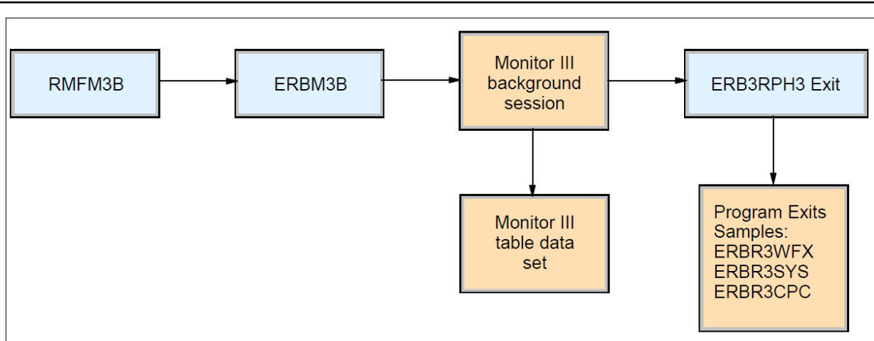
Figure 49. RMF Monitor III batch reporter workflow diagram
