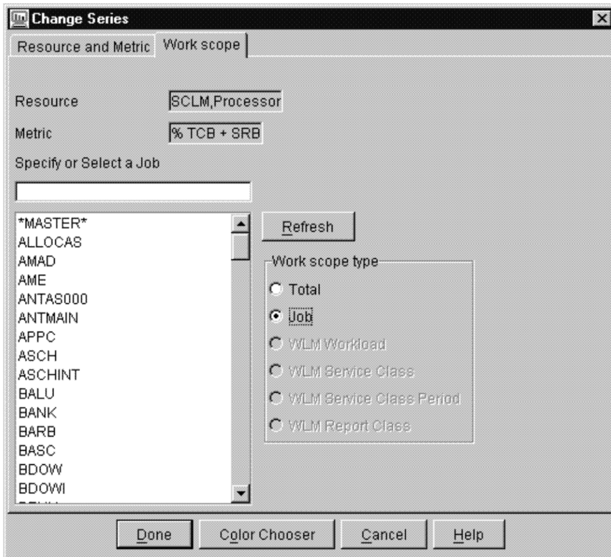
Figure 77. Work Scope Dialog
