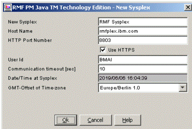
Figure 73. Sysplex Dialog
